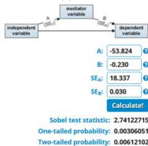
Figure 2 Sobel Test 1
